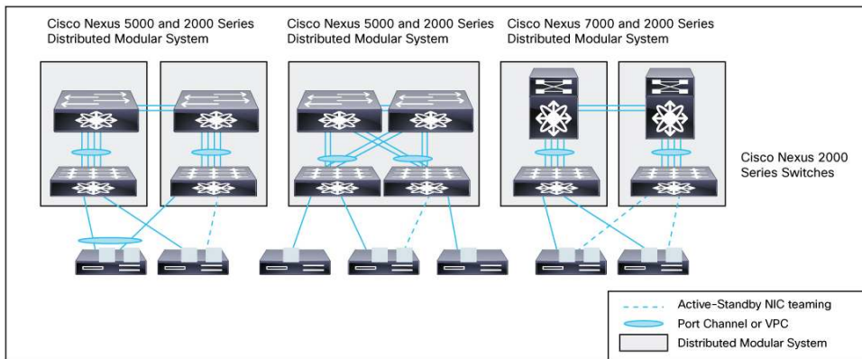
Figure 3. Cisco Nexus 2000 Series Fabric Extenders Design Scenarios, from Left to Right: Cisco Nexus 2000 Series Single Connected to One Upstream Cisco Nexus 5000 Series Switch, Cisco Nexus 2000 Series Dual-Connected to Two Upstream Cisco Nexus 5000 Series Switches, and Cisco Nexus 2000 Series Single-Connected to One Upstream Cisco Nexus 7000 Series Switch
